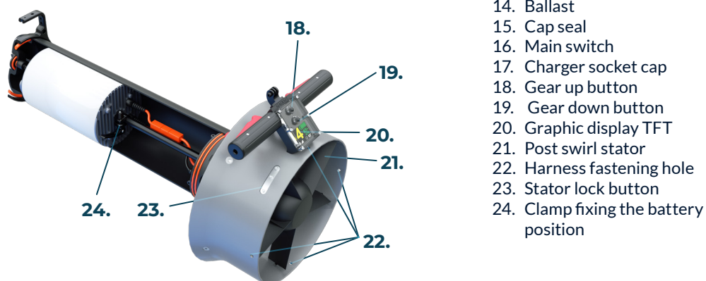
Figure 4 Overview of the basic components of the scooter
